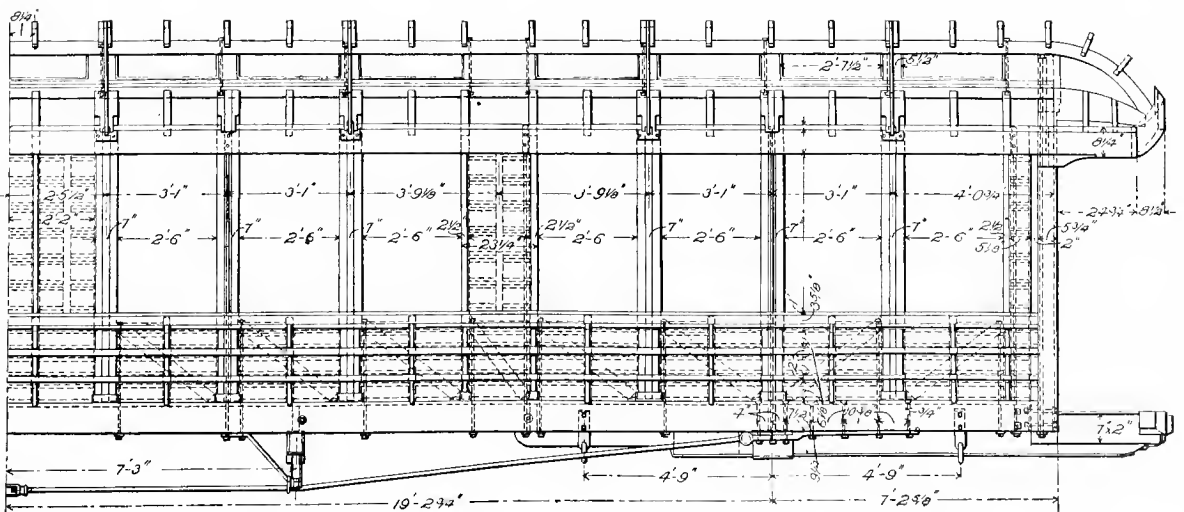
Fig. 493. Half Side Elevation of Framing.
